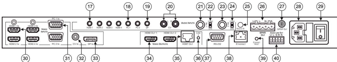
Figure 2: VP-773AMP Presentation Switcher/Scaler Rear Panel
