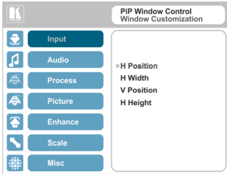
Figure 16: Window Customization
