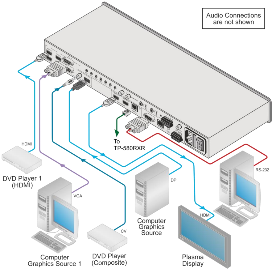
Figure 4: Connecting the VP-773AMP Presentation Switcher/Scaler
