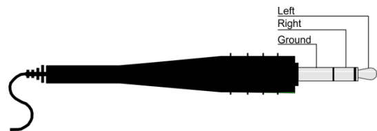
Figure 9: Audio Input Pinout
