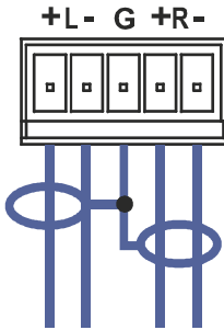
Figure 6: Connecting the Balanced Stereo Audio Output
