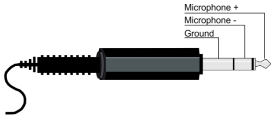
Figure 8: Microphone Pinout
