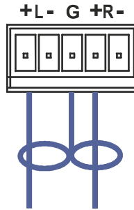
Figure 7: Connecting an Unbalanced Stereo Audio Acceptor to the Balanced Output
