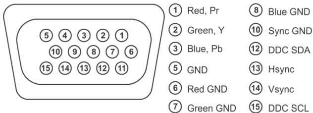
Figure 3: 15-pin HD Connector Pinout
