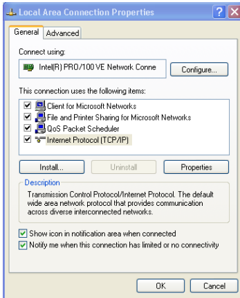
Figure 30: Local Area Connection Properties Window
