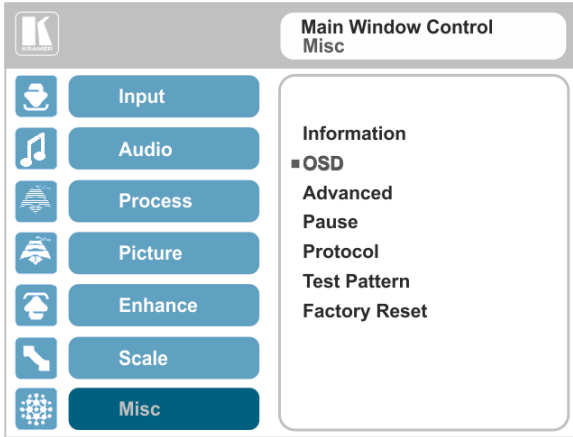
Figure 25: Misc Menu
