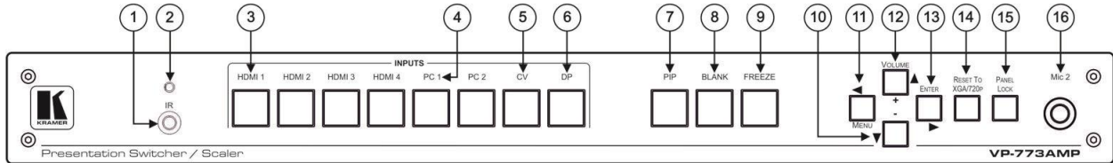
Figure 1: VP-773AMP Presentation Switcher/Scaler Front Panel
