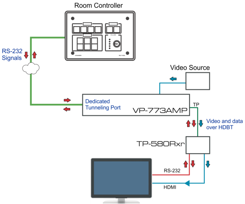
Figure 33: Port Tunneling
