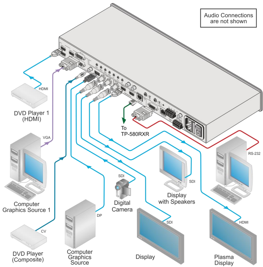
Figure 4: Connecting the VP-774AMP Presentation Switcher/Scaler
