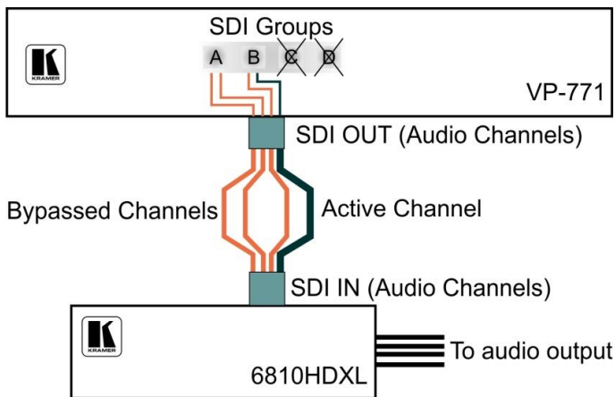
Figure 21: SDI Channelling Example
