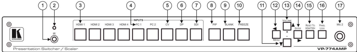
Figure 1: VP-774AMP Presentation Switcher/Scaler Front Panel
