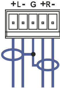
Figure 6: Connecting the Balanced Stereo Audio Output
