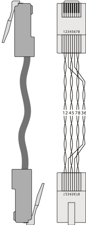
Figure 5: TP PINOUT
