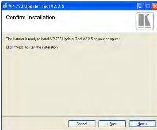
Figure 20: Confirm Installation
