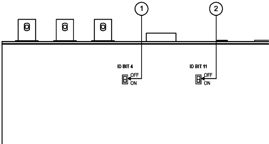
Figure 2: VP-100A Underside
